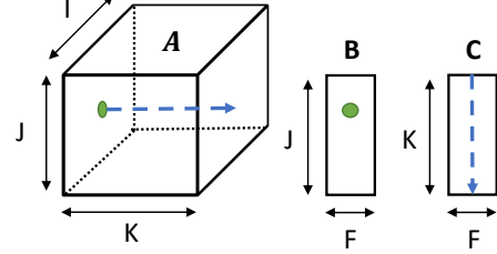
Figure 1: MTTKRP
